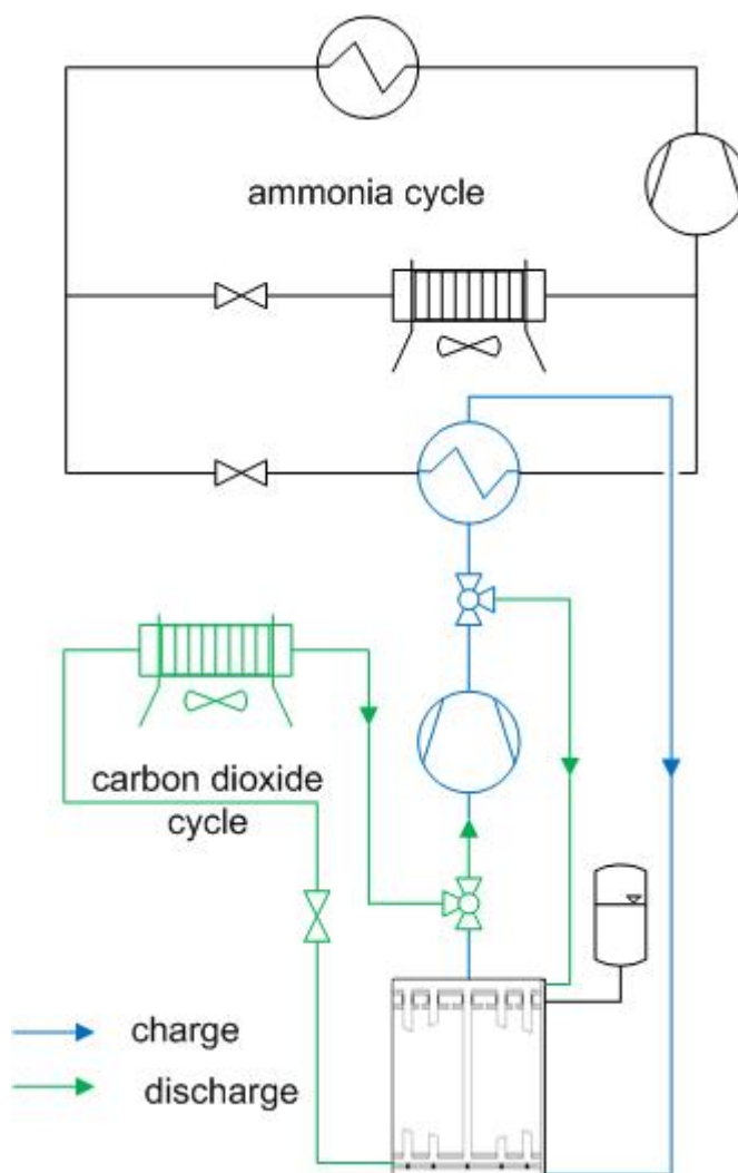
Figure 3.1: schematic of cascade process
